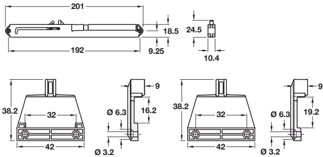
Follower for single-walled drawer side runner systems, thickness 16 and 19 mm
