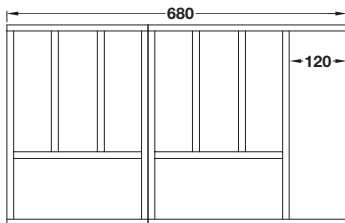
To suit 800 mm width drawer*
