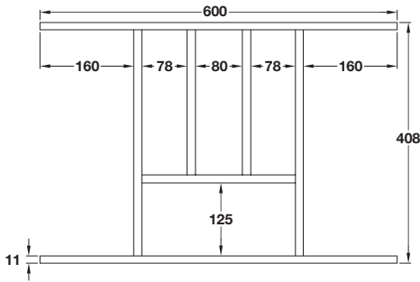
Wooden cutlery insert
