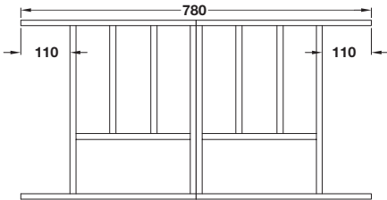
To suit 900 mm width drawer*
