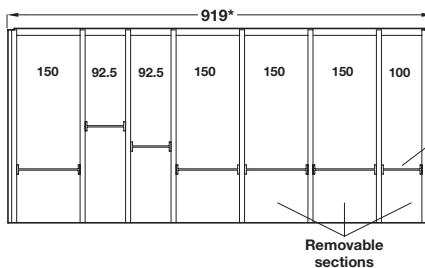
For 1000 mm drawer width (For 900 mm drawer width remove 100 mm wide section)
