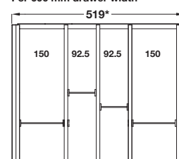
For 600 mm drawer width
