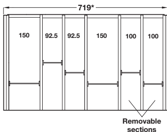
For 800 mm drawer width
