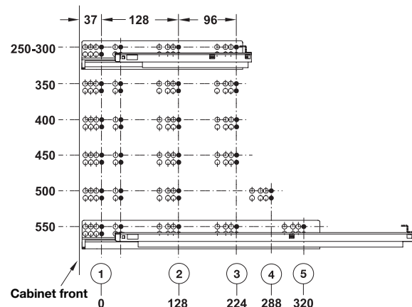
Drilling pattern
