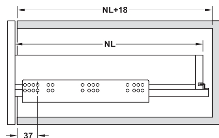
Drilling pattern
