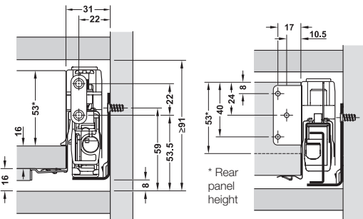
Internal installation height with Push-to-Open Soft-Close
