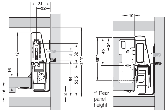
Internal installation height with Push-to-Open Soft-Close
