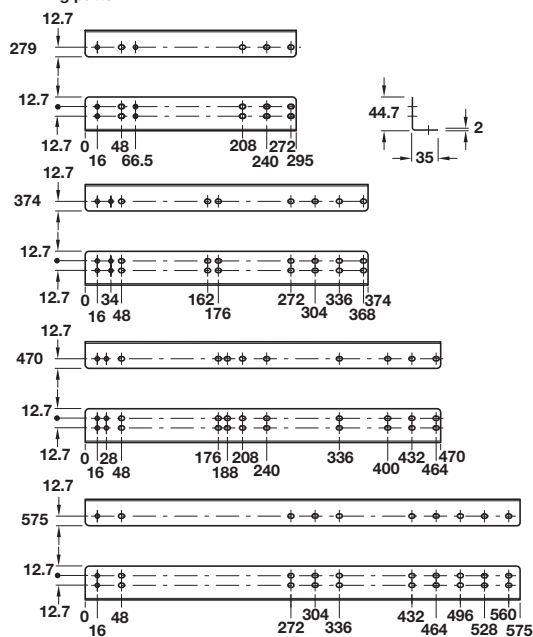
Drilling pattern
