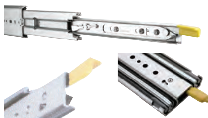
Front lever lock release
