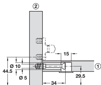
Connecting bolt
