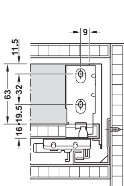
Rear panel installation dimensions
