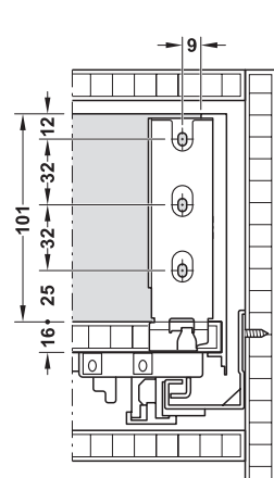
Rear panel installation dimensions
