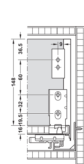
Rear panel installation dimensions
