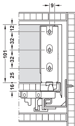
Rear panel installation dimensions
