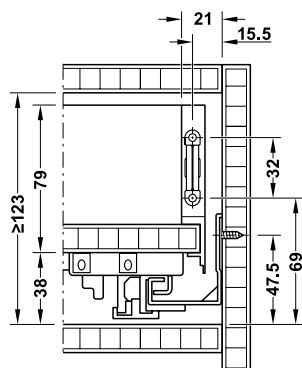
Internal installation height
