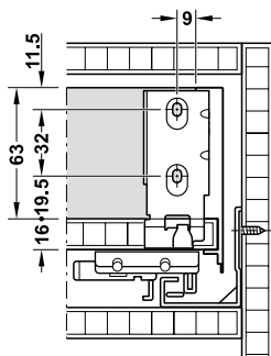
Rear panel installation dimensions
