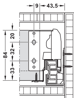
Rear panel installation dimensions
