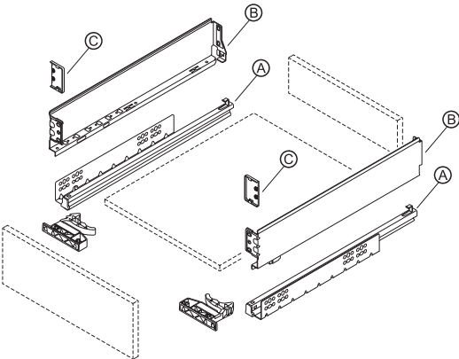
A Cabinet runner B Single-wall drawer sides C Cover caps
