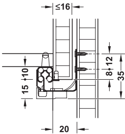
Drilling pattern
