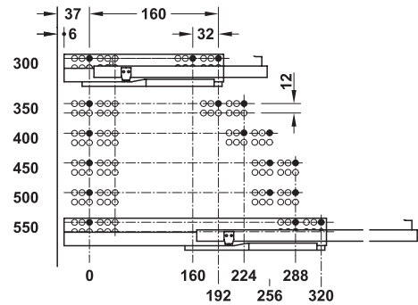
Drilling pattern
