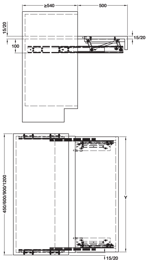
OPLÀ Pull out worktop, aligned with shelf
