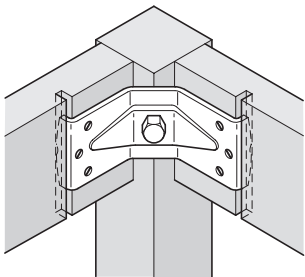
Leg screw fixed through centre hole of corner brace Table frame grooved to accept corner brace
