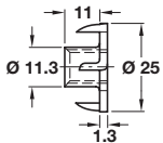
M10 internal thread
