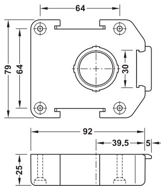
Rectangular, for screw fixing
