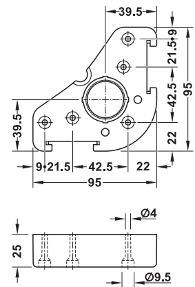
Triangular, for screw fixing
