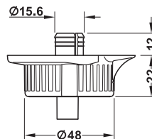
Round with lug, for press fitting
