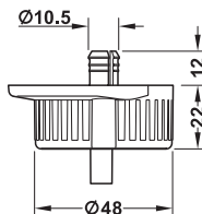
Round, for press fitting
