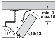
Mounting the front plinth panel with plinth spring (order separately)
