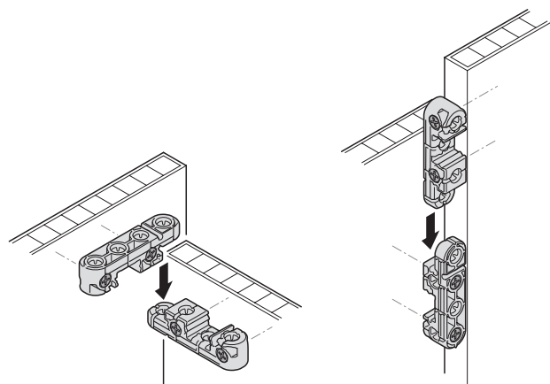
Hooked in, connection stabilised by snap in points
