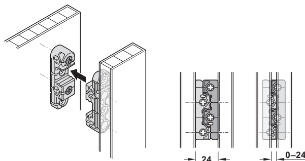
Clip on (re-release using clip spring), screw fixing or recess mounted
