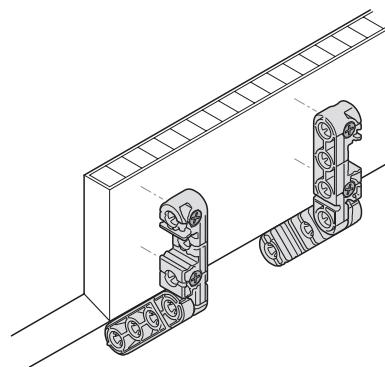
Secure connector pairs against lateral movement by reversed mounting
