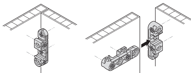
Screw fixed, e.g. for corner connections
