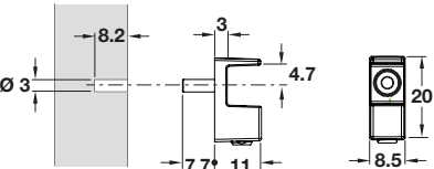
For 8 mm glass thickness
