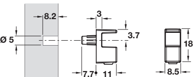
For 5-6 mm glass thickness
