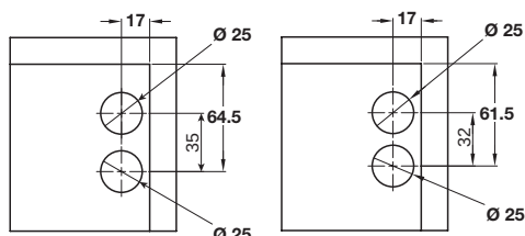
Rear drilling pattern for active safety version. Two possibilities.
