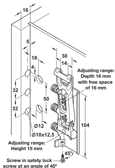
Hook-off protection
