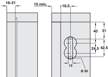
Drilling plan for both rectangular and round cover caps shown on page 81
