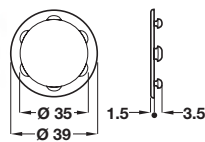
Round cover cap for Ø 35 mm hole
