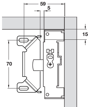
Wall plate position with SH bracket
