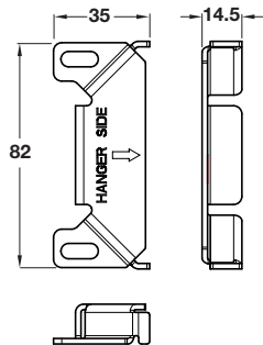
Wall plate position with SH bracket
