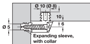
For single-sided installation - Hospa pan head screw 015.71.679 and expanding sleeve, with collar
