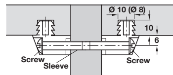
For double-sided installation - M4 threaded screw 022.35.234 and sleeve shown below
