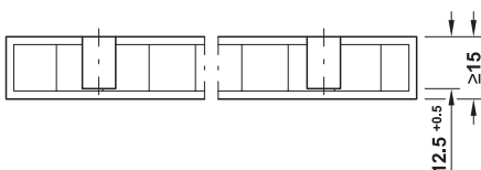
Drilling pattern
