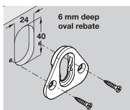
Ø 4.5 mm csk screws for rebated option
