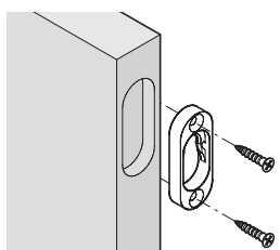
22 x 56 x 8 mm oval rebate Ø 4.5 mm countersunk screws
