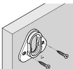
Ø 5 mm pan head screws for surface-mounted option
