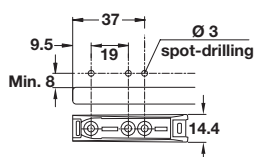
Surface mounted - short
