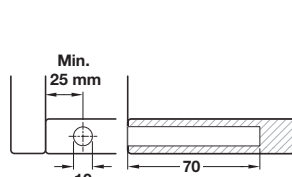
Recess mounted - long
