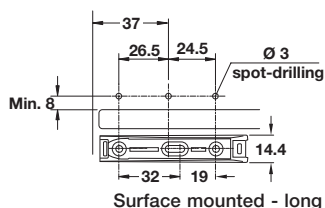
Surface mounted - long
