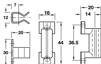
Spring catch
