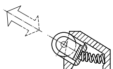
Closing mechanism: linear-action roller
