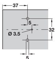
With pre-mounted Euro screws
