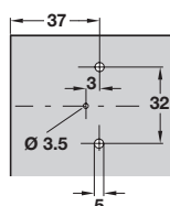
For Varianta screws
