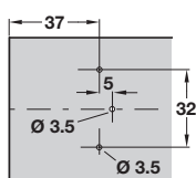
For Hospa screws
