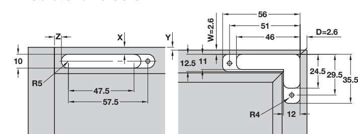
Installation dimensions
