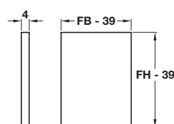
Glass dimensions
