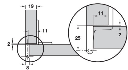
Screw mounting
