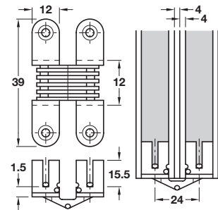
Concealed hinge, maximum door thickness 18-20 mm
