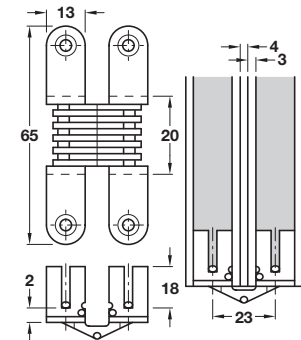
Concealed hinge, maximum door thickness 19-21 mm
