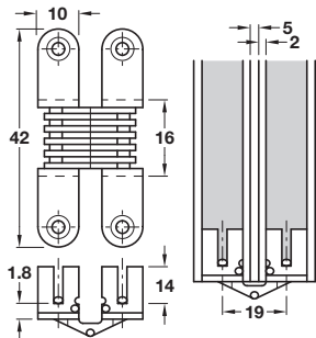
Concealed hinge, maximum door thickness 14-16 mm
