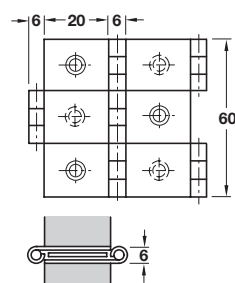
For 20 mm door/side thickness
