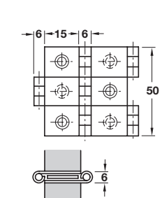
For 15 mm door/side thickness
