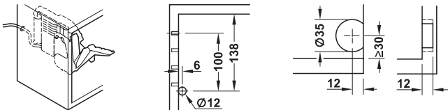
Push button sender and cable guide installation
