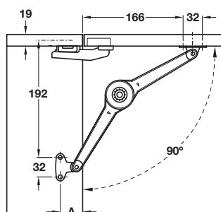
Installation as flap stay
