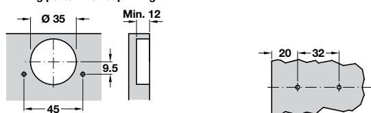
Drilling pattern for cup fixing
