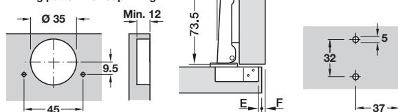
Drilling pattern for cup fixing
