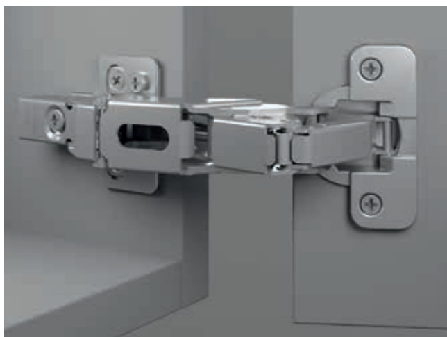
Full overlay mounting with mounting plate
