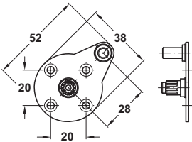
Drilling pattern
