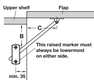
Front-hung flap
