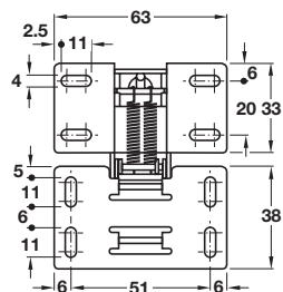
Adjustment facility - Holding power adjustable with screwdriver
