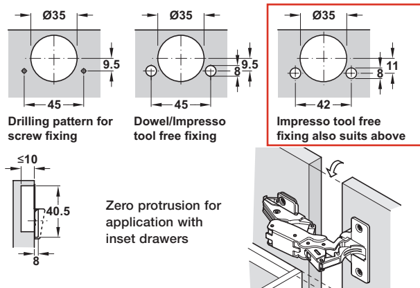
Drilling pattern for cup fixing
